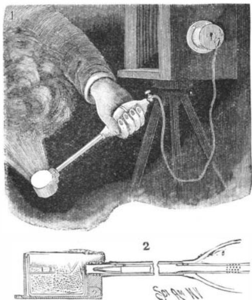
MALICK'S FLASH LIGHT APPARATUS.
