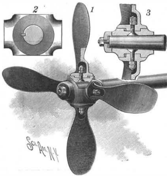
DAVIES' PROPELLER.
