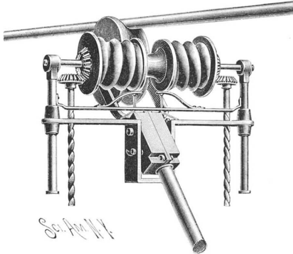
JONES' TROLLEY WIRE FINDER.
