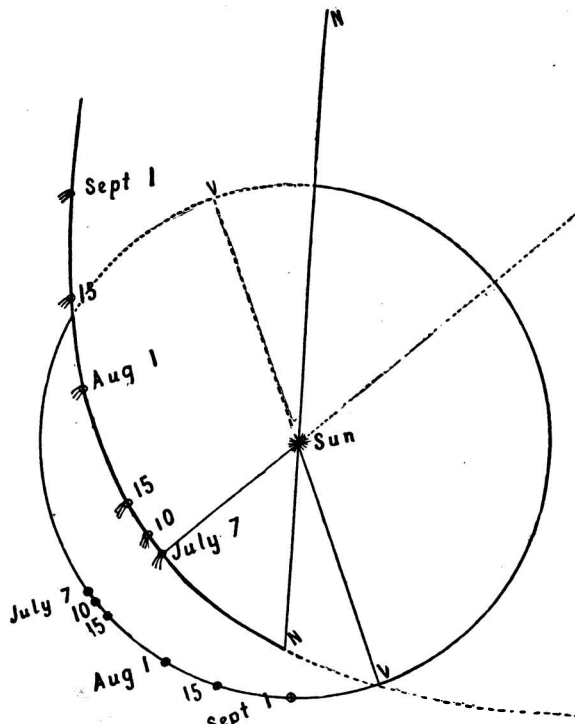
DIAGRAM SHOWING RELATIVE POSITIONS OF COMET β 1893 AND THE EARTH.
