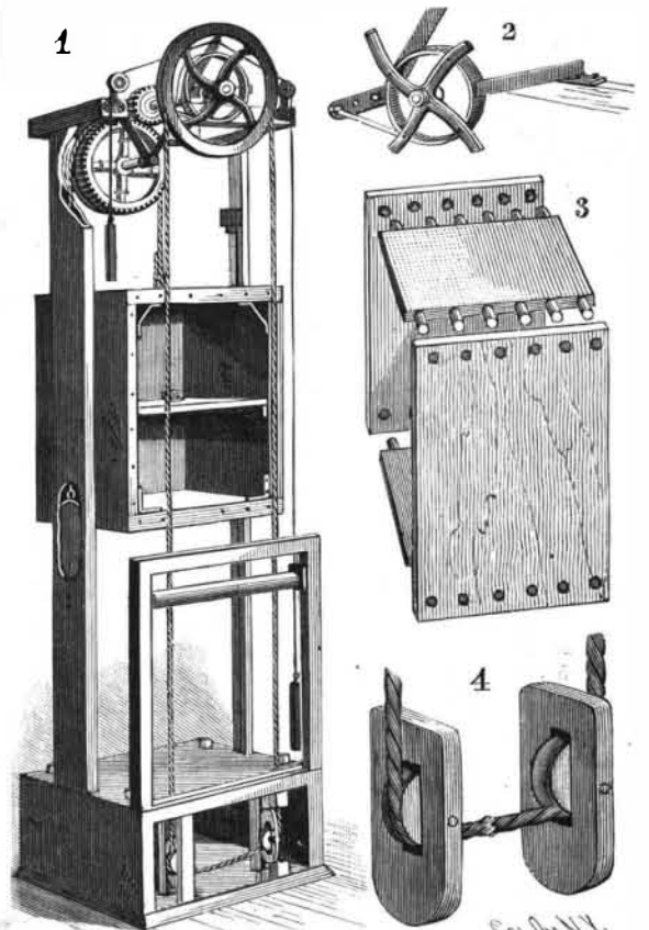
LARSEN'S DUMBWAITER.
