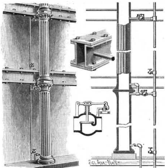
WILLIAMS' APPLIANCES FOR COOLING IRON STRUCTURES.
