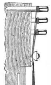
STRINGING-OLD METHOD.
