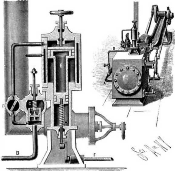
MCIHENNY'S STEAM ENGINE GOVERNOR.
