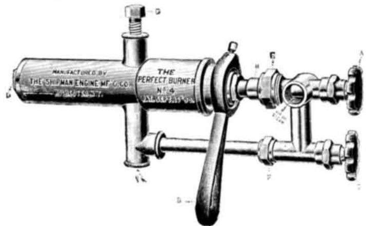
AN IMPROVED CRUDE OIL BURNER.
