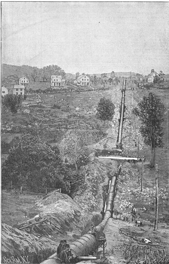
LAYING THE CONDUIT UNDER STONE HOUSE BROOK.
