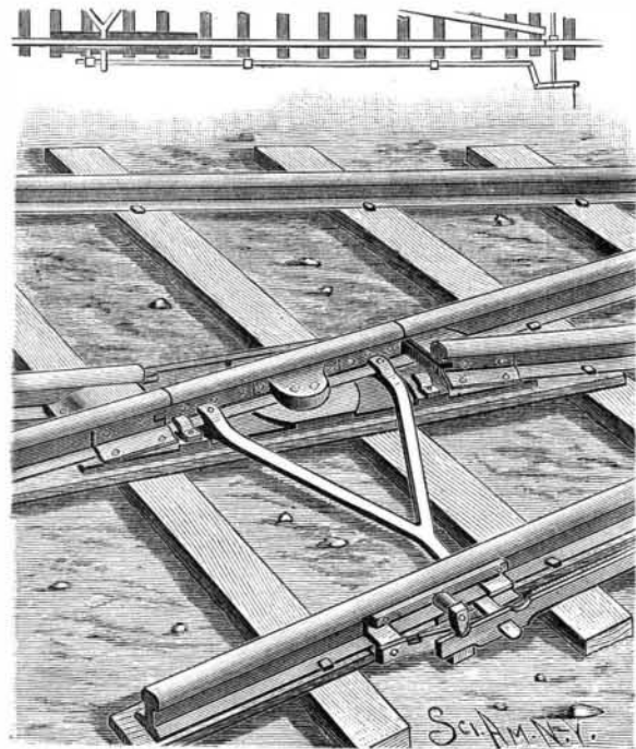
BAIRD'S IMPROVED RAILROAD FROG.
