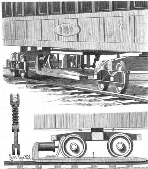
DIEDEL'S BRAKE SHOE.
