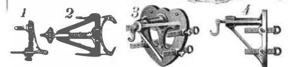
PRITCHARD'S HAMMOCK SUSPENSION DEVICE.
