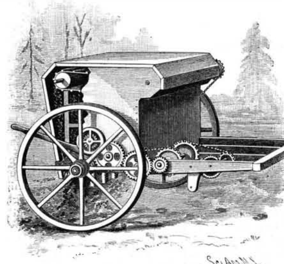
GREAVES' "SHAKER" FERTILIZER DISTRIBUTER.
