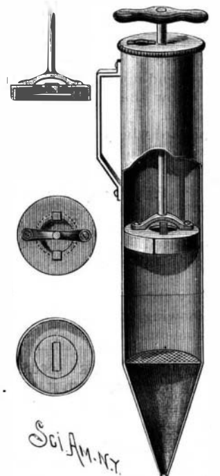
LOUGHRY'S FUMIGATOR.
