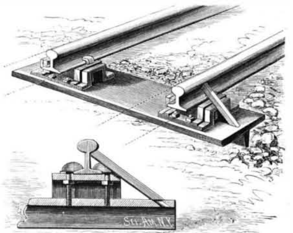
MOSER & MOECKEL'S RAILWAY TIE.
