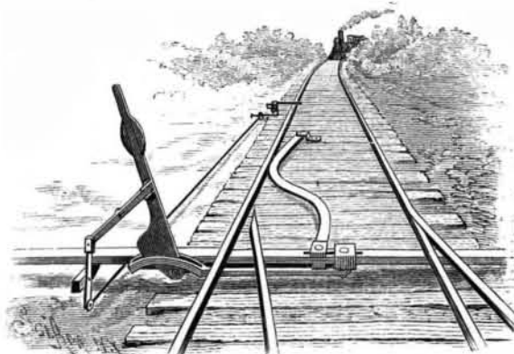
SUFFERN'S RAILWAY SWITCH. [FOR DESCRIPTION SEE PAGE 275.]
