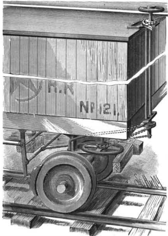
QUATERMASS' CAR BRAKE ATTACHMENT.
