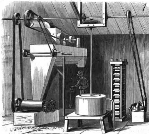
BAUMGARTEN'S APPARATUS FOR EXTRACTING OIL FROM SEEDS.
