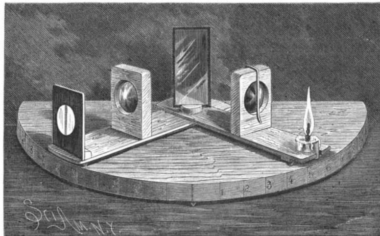
APPARATUS FOR ILLUSTRATING THE LAW OF THE REFLECTION OF LIGHT.
