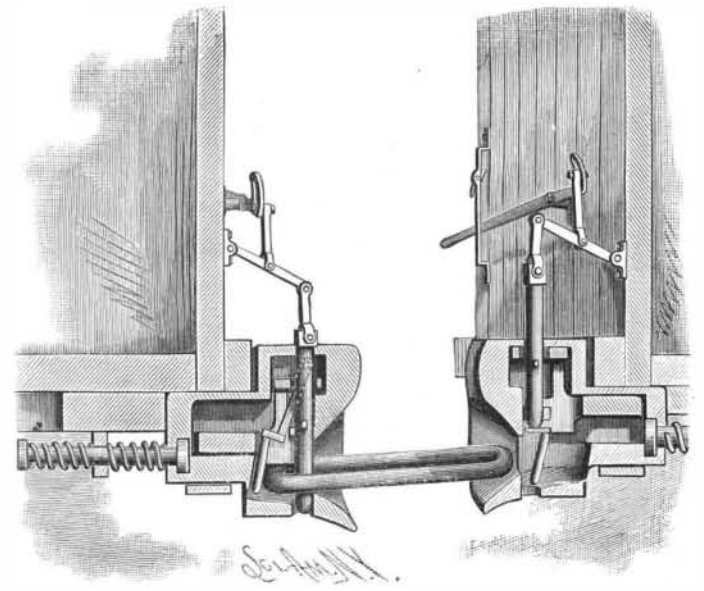
THE KEYSTONE AUTOMATIC CAR COUPLER.
