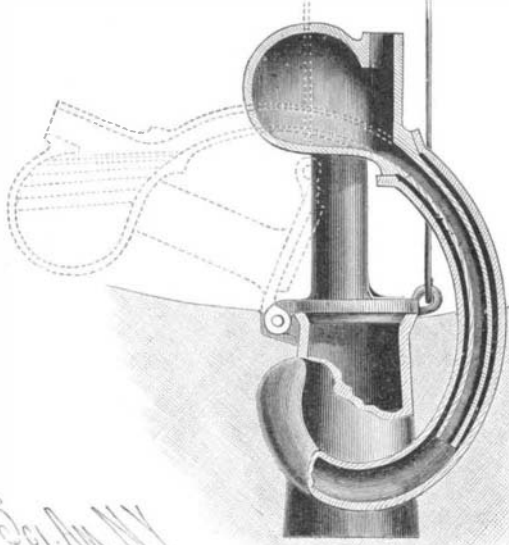
BEARD'S DISCHARGE PIPE FOR VAULTS.
