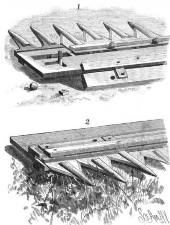
VOSS' CUTTING APPARATUS FOR MOWERS AND REAPERS.
