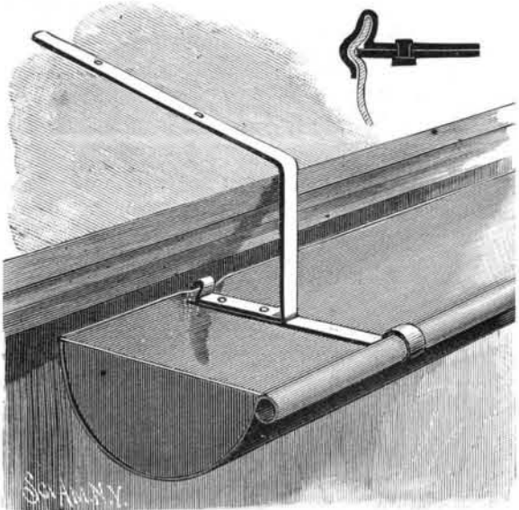
HOEPFNER'S EAVES-TROUGH HANGER.
