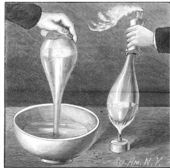
EXPERIMENT IN CONDENSATION OF STEAM.
