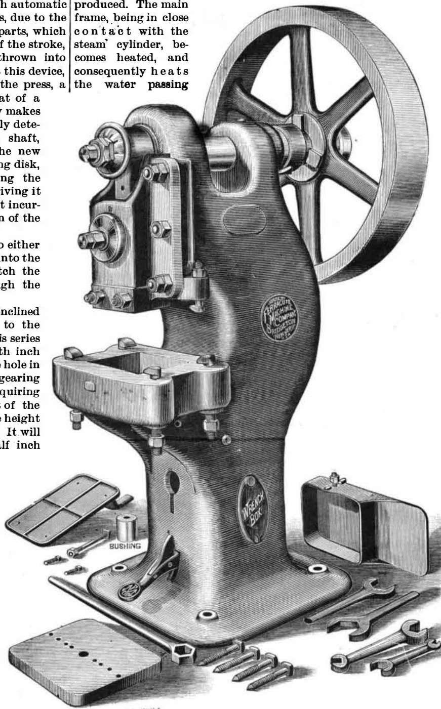
NEW POWER PUNCHING PRESS.
