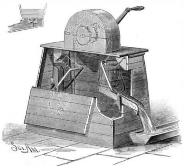
DAVIS' IMPROVED WATER ELEVATOR.
