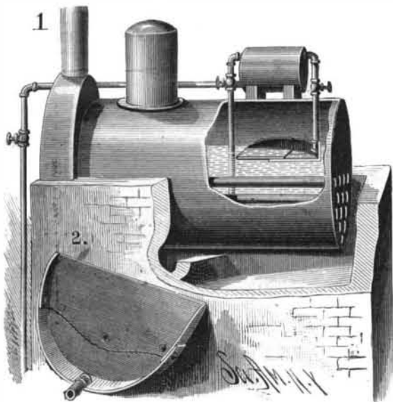
ESTELLE'S BOILER CLEANER.
