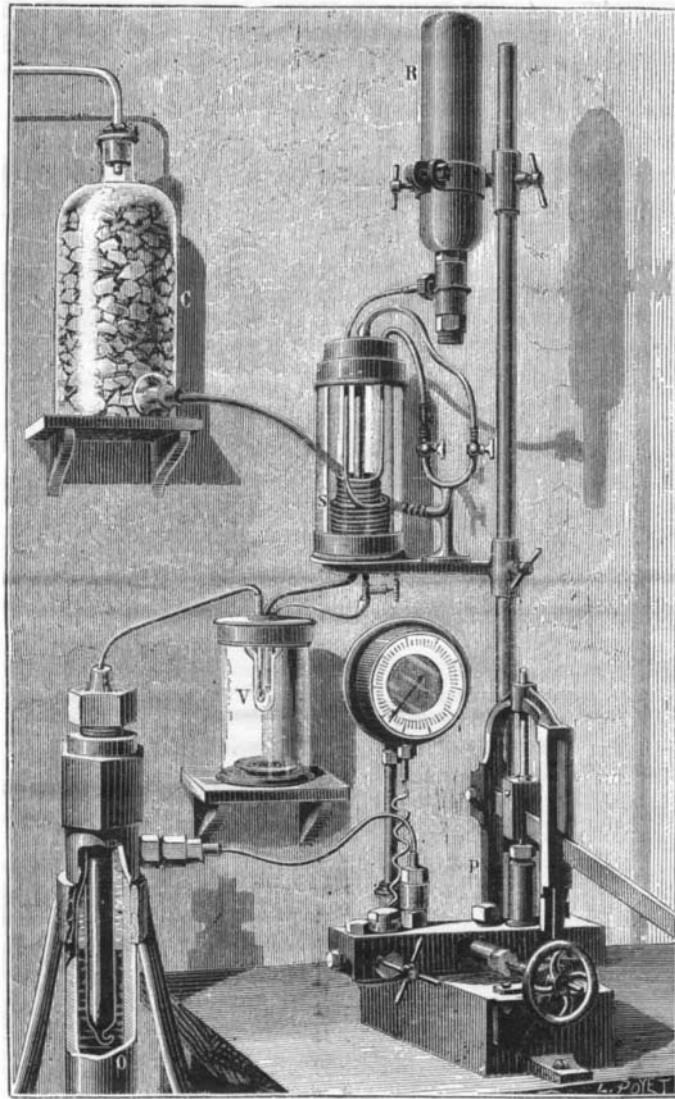
CAILLETET'S APPARATUS FOR LIQUEFYING OXYGEN.
