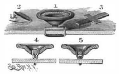
IRVINE'S BUTTON FASTENER.
