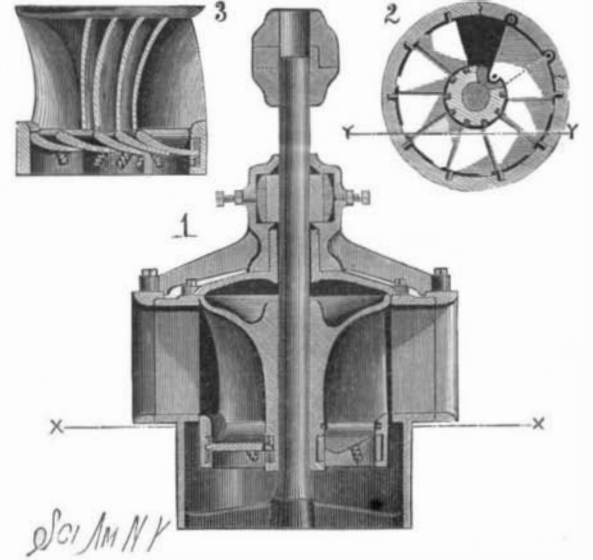
TRULLINGER'S GATE FOR WATERWHEELS.
