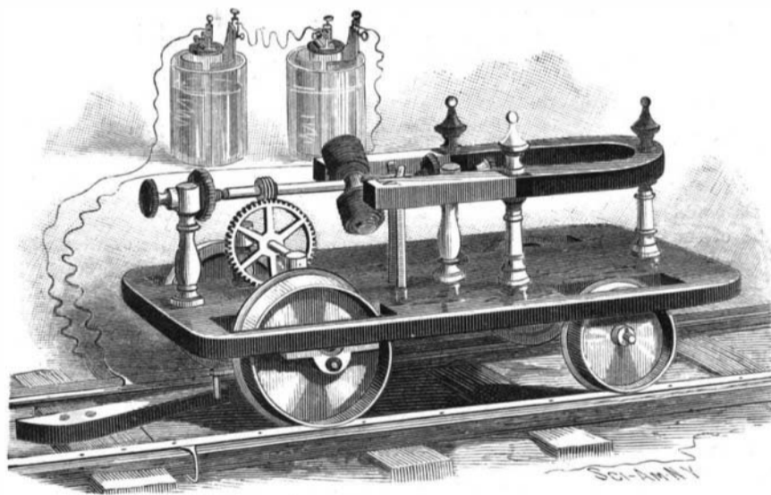
Fig. 1.—ELECTRO-MAGNETIC LOCOMOTIVE.
