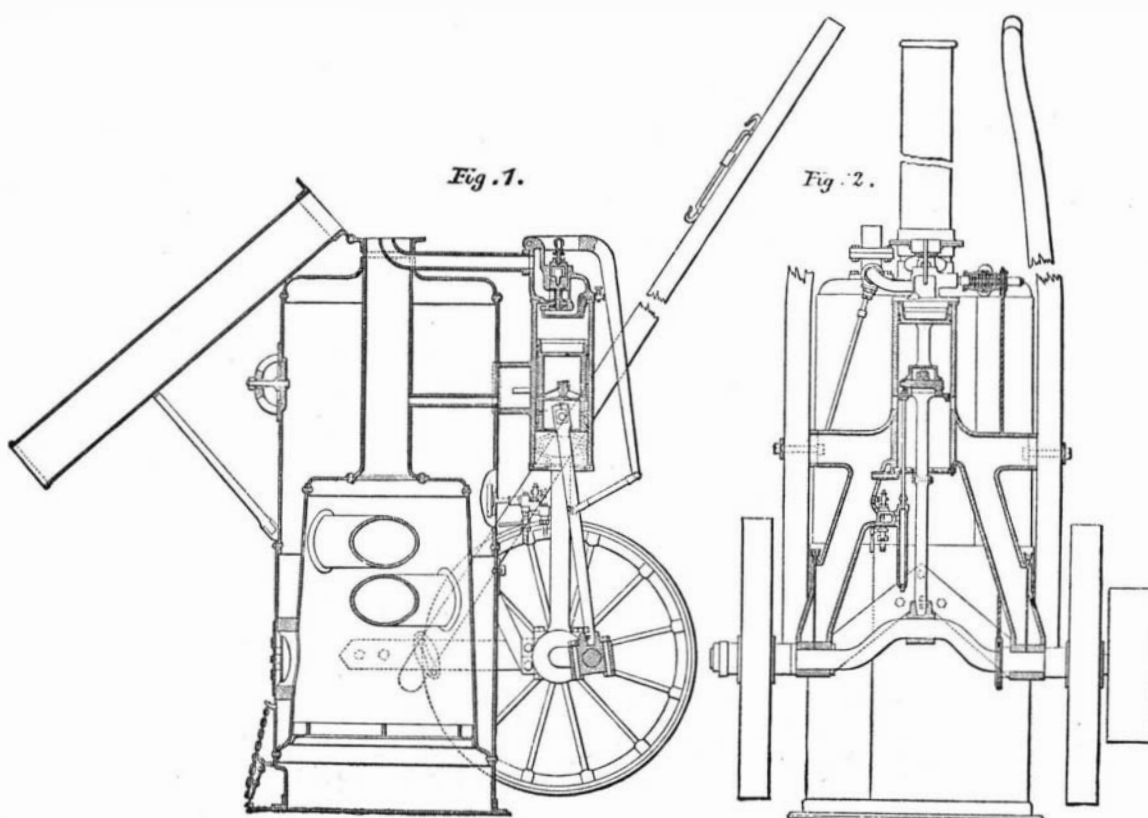
IMPROVED PORTABLE ENGINE.
