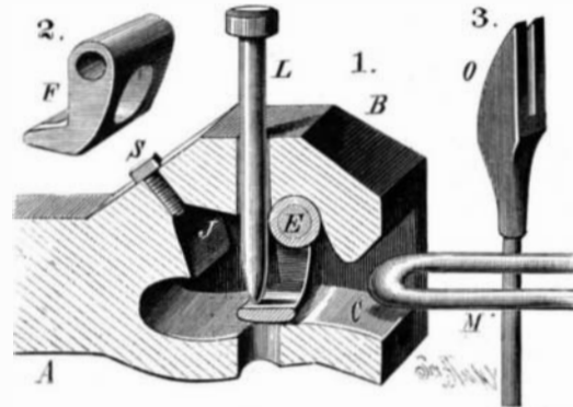
NICHOLAS' IMPROVED CAR COUPLING.
