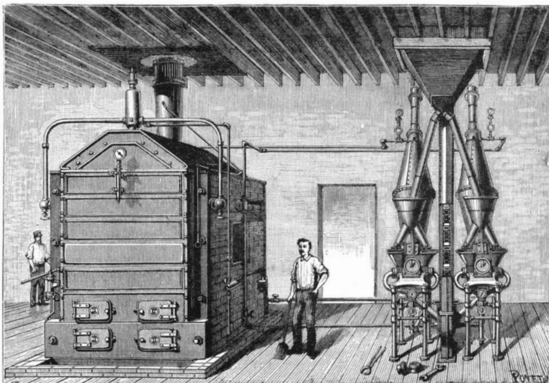
Fig. 1.—PNEUMATIC PULVERIZER.
