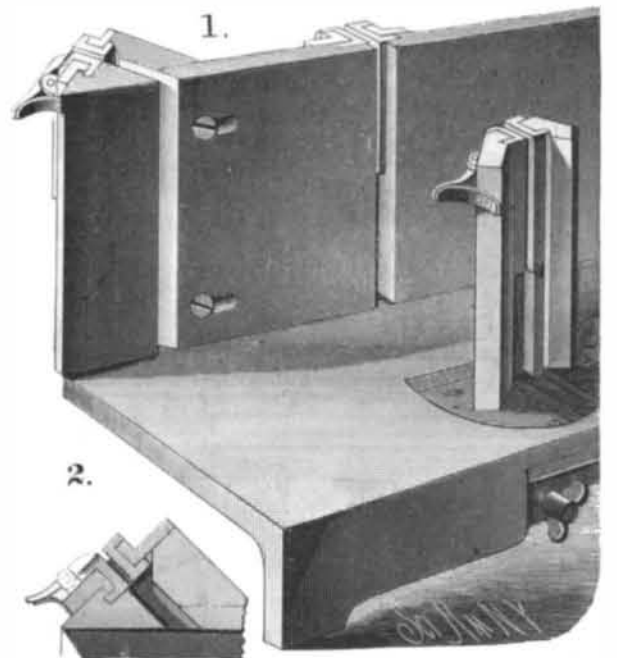
CASHIN'S MITER BOX.
