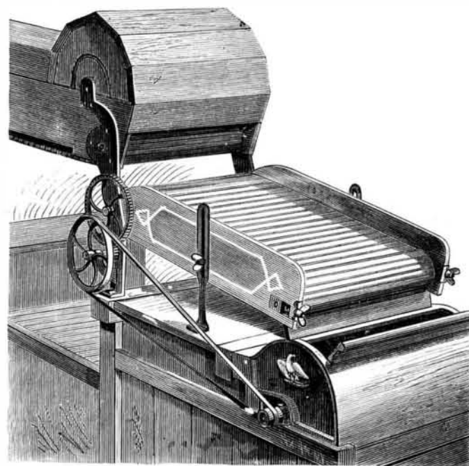
STIETENROTH'S FEEDER FOR COTTON GINS.
