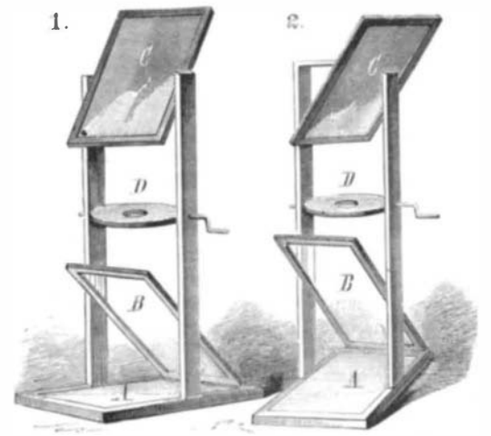
POLARIZING APPARATUS
