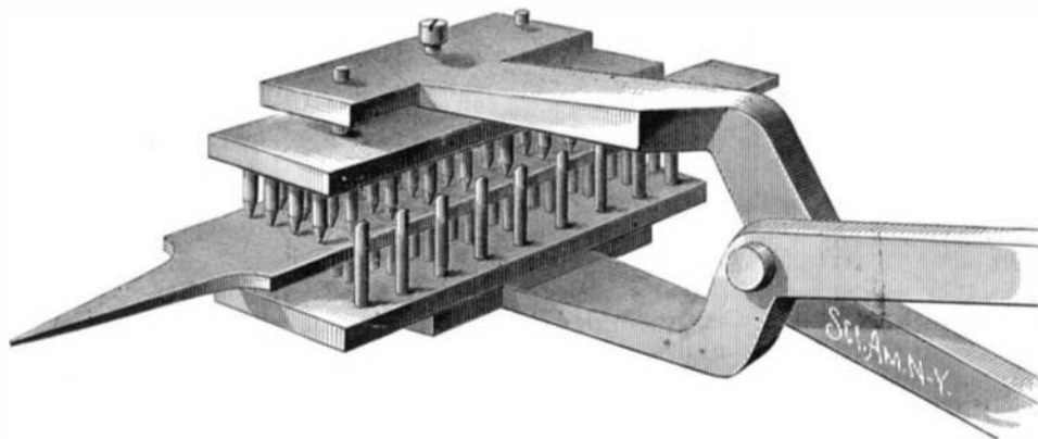
HARDENING TONGS.
