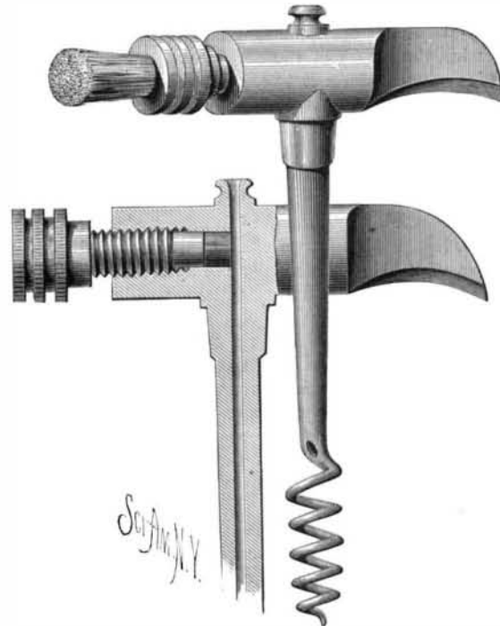
LANT'S COMBINED CORKSCREW AND BOTTLE FAUCET.
