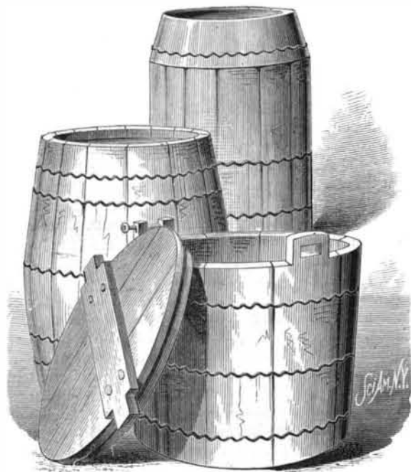
EISELEIN'S CORRUGATED HOOP FOR BARRELS.
