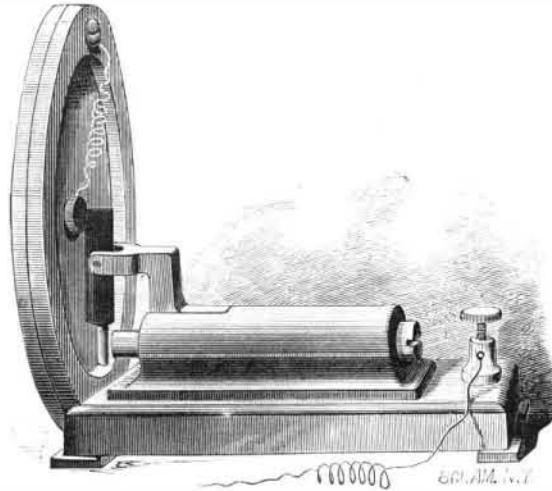
DOWLING'S IMPROVED MICROPHONE.
