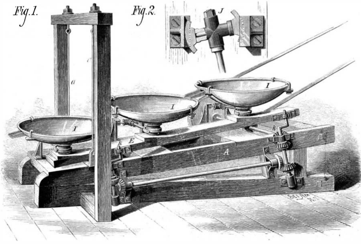
PECK'S AMALGAMATOR.
