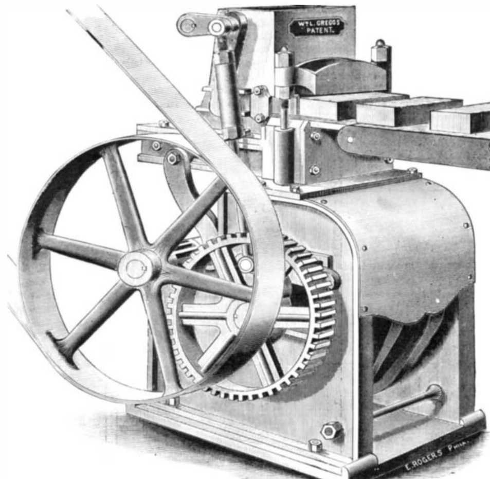
GREGG'S BRICK MAKING AND REPRESSING MACHINE.
