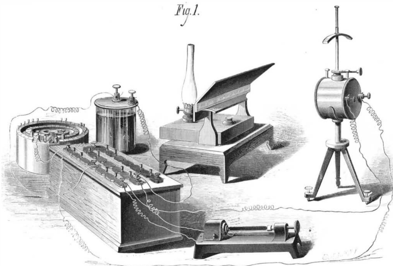
EDISON'S MICRO-TASIMETER.
