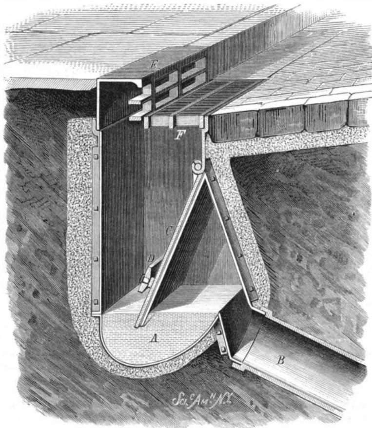
DARK'S CAST IRON RECEIVER AND STENCH TRAP.
