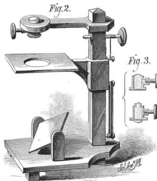
WATER LENS MICROSCOPE COMPLETE.
