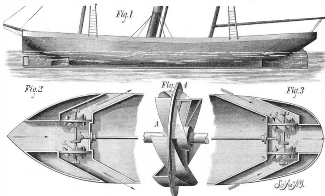
CURTIS' IMPROVED PROPELLER.
