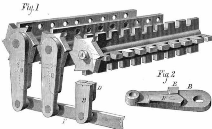
DENNY & RUTH'S IMPROVED GRATE BAR.
