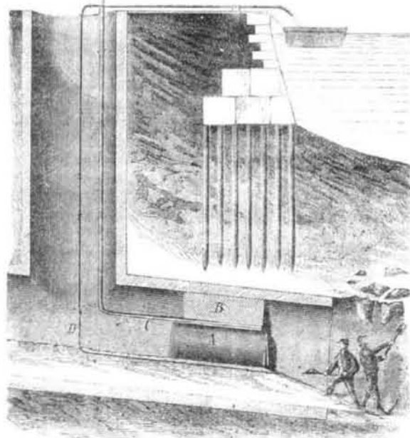
HASKIN'S NEW ART OF TUNNELING.
