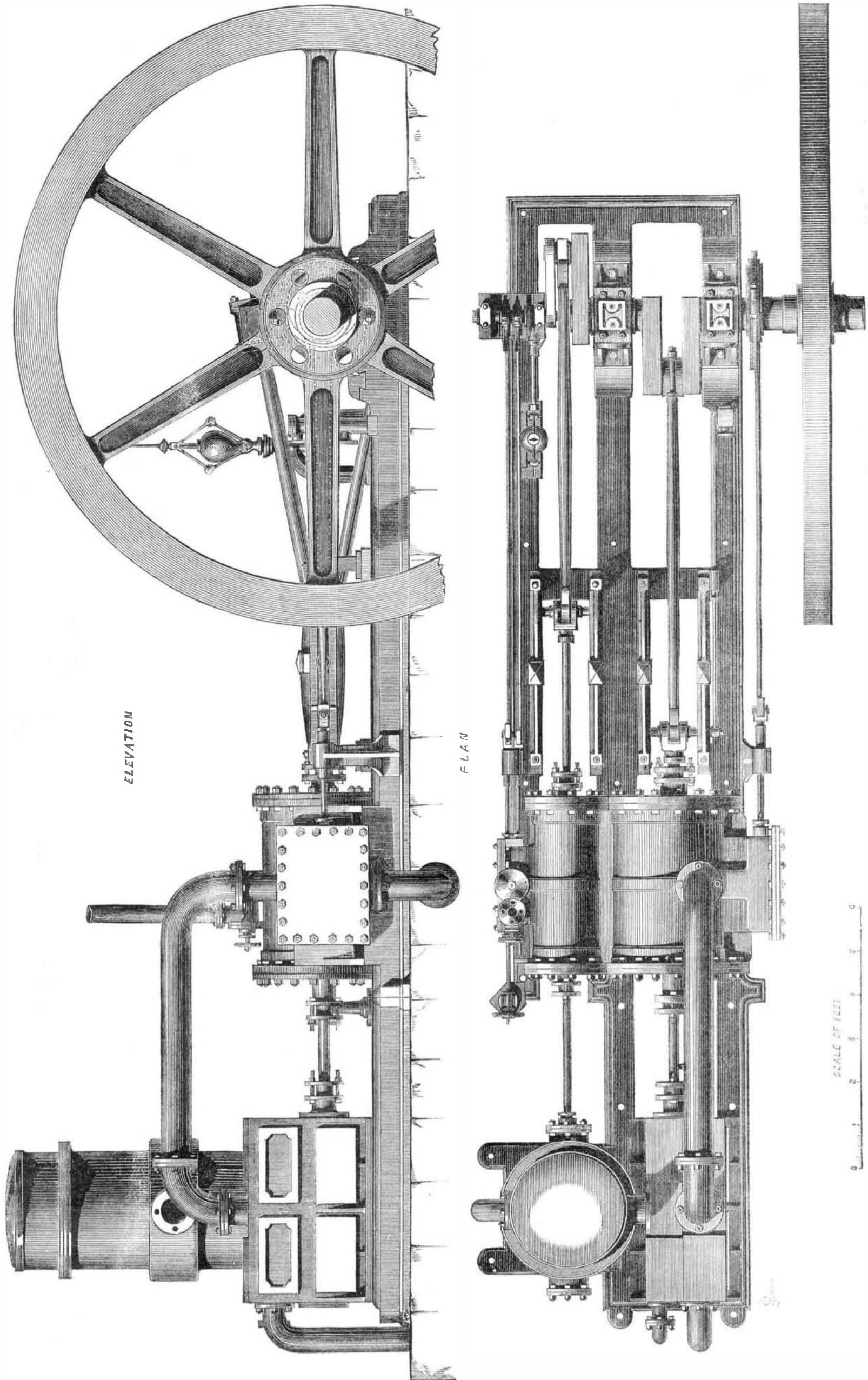
HATHORN & CO'S HORIZONTAL COMPOUND ENGINE.
