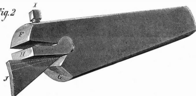
EMERSON'S PLANER-TOOTHED SAW AND ADJUSTABLE SWAGE.
