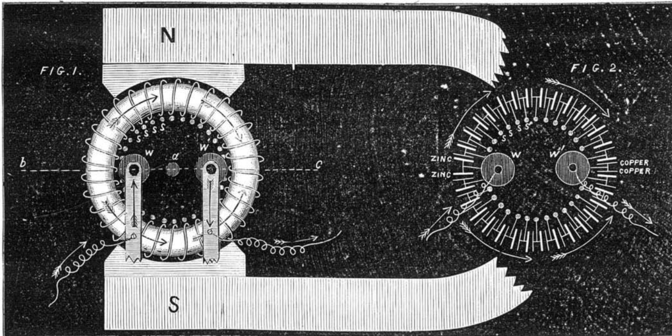
MAGNETO-ELECTRIC MACHINE.
